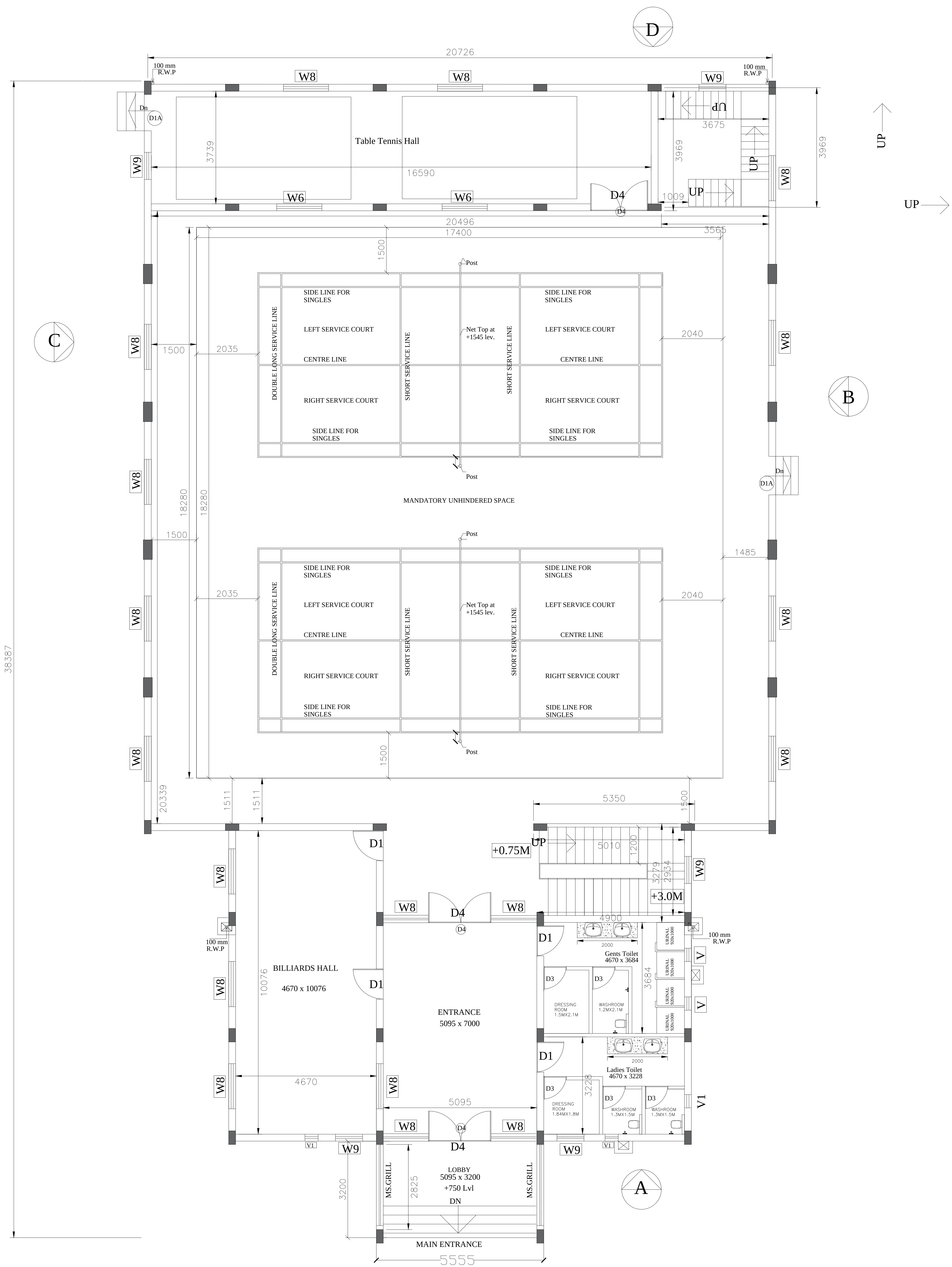
PLAN AT +750mm LVL
